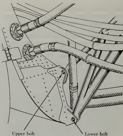
FIGURE 8-22. Engine mount attachment point.
